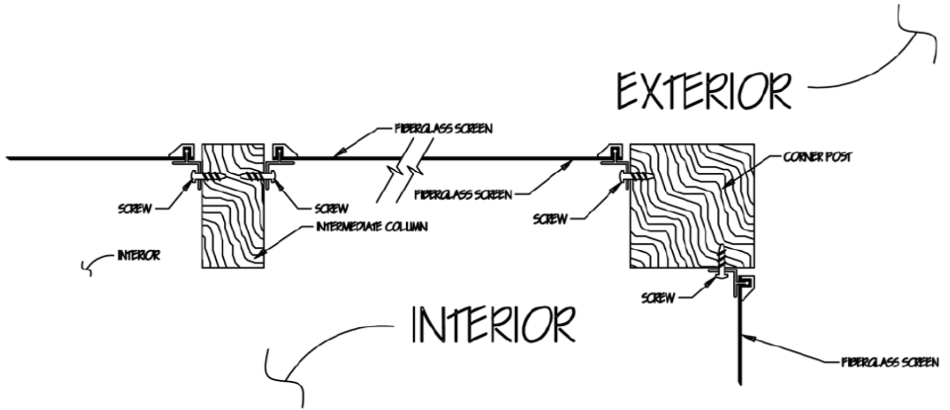
FLUSH MOUNT EXTERIOR DETAIL
